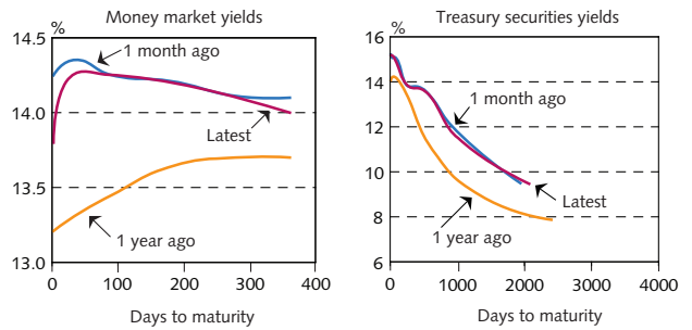
Term structure of nominal interest rates Sept. 21, 2007
