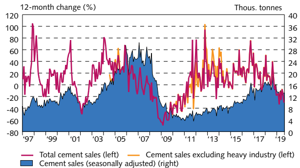
Cement sales
