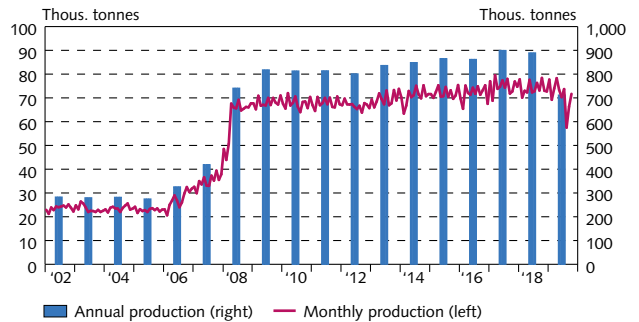
Aluminium production
