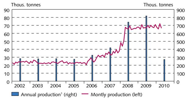
Aluminium production
